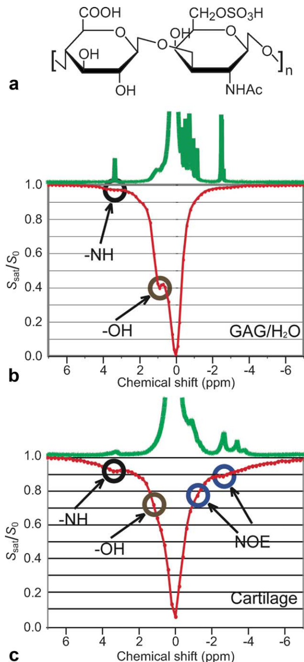
FIG. 5. Z-spectra for glycosaminoglycans (gags) in solution and in cartilage showing CEST and cross-relaxation effects (PBS, 11.7 T, t_{\text{sat}} = 4 s, 2.35 \mu\text{T} , 37^\circ\text{C} ). a: structure of gag-unit, showing three OH groups, an amide proton and several aliphatic protons in the ring (CH) and the N -Acetyl side chain. b: Z-spectra of 125 mM gag units in solution, showing predominantly NH and OH exchange saturation transfer effects. c: Z-spectra of cartilage from bovine patella in PBS buffer showing exchange and much increased cross-relaxation [nuclear Overhauser enhancement (NOE)] effects. Reproduced with permission from Ling et al., Proc Natl Acad Sci USA 2008;105:2266–2270. [Color figure can be viewed in the online issue, which is available at wileyonlinelibrary.com .]
