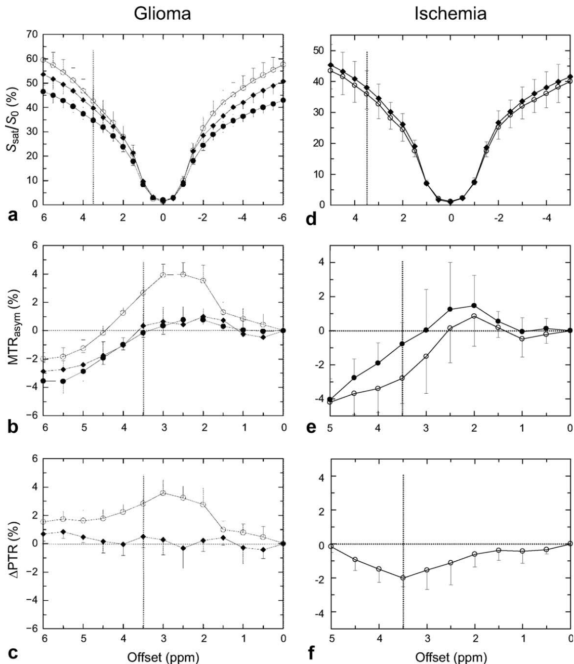
FIG. 7. Effect of MTC on Z-spectra and CEST data analysis for 9L glioma (a–c) and ischemia (d–f) in rat brain (Multipulse saturation: 400 gaussian 180° pulses, 4.7 T, t_{\text{sat}} = 4 s, B_1 = 1.2 \mu\text{T} ). Solid circle: contralateral brain; diamond: peritumoral tissue (a–c); open circle: tumor (a–c) or ischemic lesion (d–f). Signal attenuation in Z-spectra (a, d) is due mainly to direct water saturation close to the water frequency and a large MTC effect (40 to 60%) over the whole spectral range. The MTC contribution is reduced for edema and tumor (a), indicating a higher water content for these tissues. The Z-spectra are slightly asymmetric, which becomes visible when performing asymmetry analysis (b, e). Both exchange effects and asymmetry in the MTC contribute to the residual curve, with the latter reflected in a relatively constant negative \text{MTR}_{\text{asym}} (2–3%) at offsets above 5 ppm. The PTR for tissue changes can be estimated by comparing lesion with normal brain, removing most of the MTC effects (c, f). This shows that edematous regions can be separated from tumor (c) and ischemia from normal brain (f). The positive (c) and negative (f) PTR differences were attributed to increases in protein content and reduced pH, respectively. Reproduced with permission from Zhou et al., Magn Reson Med 2003;50:1120–1126 (a–c) and Nat Med 2003;9:1085–1090 (d–f).
