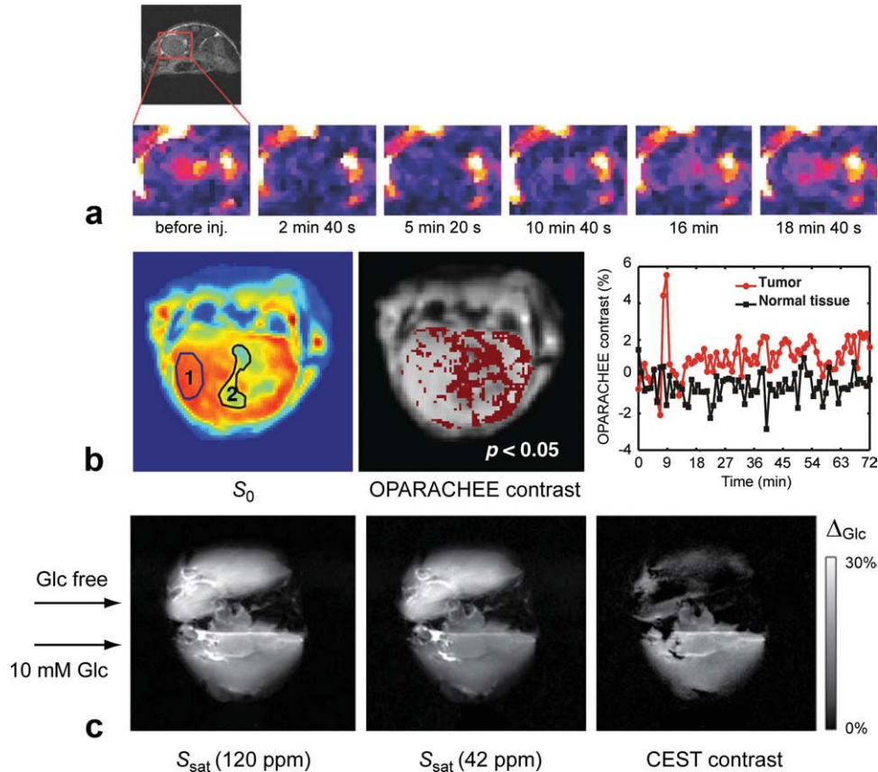
FIG. 13. In vivo and ex vivo CEST studies of molecular exchange compounds. a, b: paraCEST perfusion imaging in vivo. a: Kidney perfusion study by Vinogradov, showing CEST images before, during and after injection of Tm-DOTAM-Gly, with hypointensity when the agent reaches the kidney. Reproduced with permission from Vinogradov et al., Magn Reson Med 2007;58:650-655. b: Brain and glioblastoma perfusion study using Tm-DOTAM-Gly-Lys. Left: Flash image for region assignment of healthy tissue (1) and tumor (2). Right: Dynamic signal changes before, during and after perfusion, showing that some agent is retained in the leaky tumors, but not in brain. Middle: significantly changed CEST contrast in regions roughly corresponding to tumor. Reproduced with permission from Li et al., Proceedings of the 18th Annual Meeting of ISMRM, Stockholm, Sweden, 2010 . p 3752. c: Glucose sensing ex vivo using paraCEST agents. MRI images of two mouse livers, one perfused with Eu-D2MA-2PB solution containing glucose (Bottom) and another without glucose (Top). CEST contrast is clear in the liver perfused with glucose only. Reproduced with permission from Ren et al., Magn Reson Med 2008;60:1047-1055.
