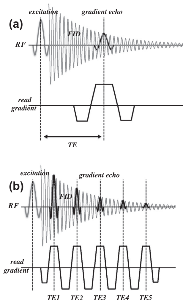
Fig. 4. (a) Basic MRI pulse sequence used for susceptibility-weighted MRI. Only RF and readout gradient are shown. After signal excitation, the FID signal is sampled with a gradient echo centered at the echo time (TE). (b) Modified pulse sequence to more completely sample the FID. Multiple echoes are sampled over a range of TE's, allowing analysis of the decay characteristics and extraction of quantitative parameters.
