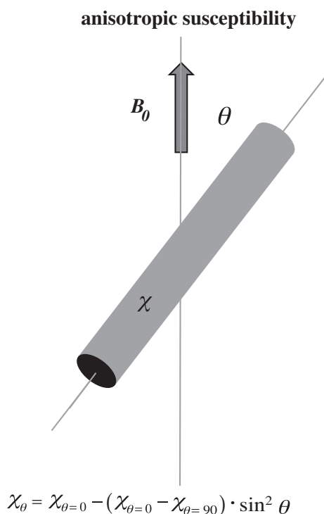
Fig. 6. Long cylindrical objects with highly organized microstructure (such as myelinated axons) may exhibit anisotropic susceptibility that has a \sin^2 \theta dependence on their angle with the magnetic field.
