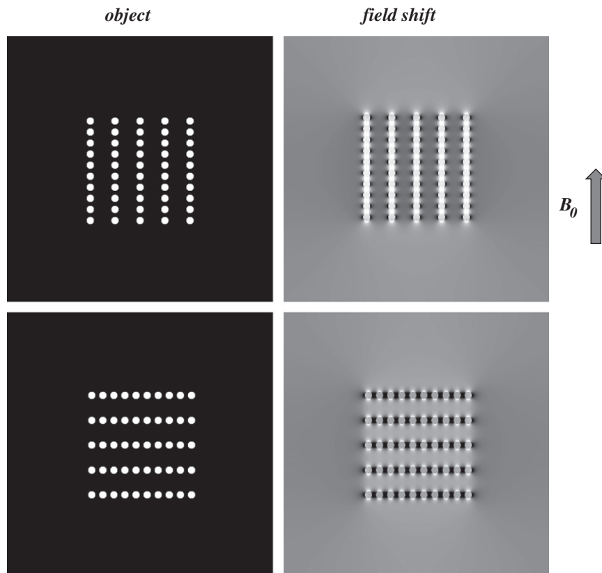
Fig. 5. Simulated dependence of field shift on object microstructure. Water molecules preferentially sample the space between the susceptibility perturbers (white), leading to a biased sampling of the magnetic field pattern and a bias in the resulting mean (voxel averaged) frequency. This bias is dependent on the distribution of perturbers, and on the orientation of the distribution pattern.
