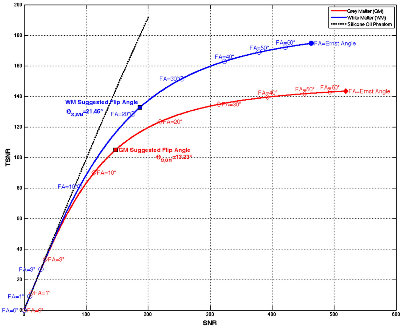
Fig. 3. Simulations of the suggested fMRI flip angle ( \theta_s ). The black dotted line shows a linear behavior for the Silicone Oil Phantom. The red and blue continuous lines show behavior for grey and white matter respectively. Ernst angle for these two tissue compartments is marked with filled dots, while other exemplary angles are marked as transparent dots. The suggested flip angle for both tissue compartments are also marked in each curve as filled squares with black outline.
