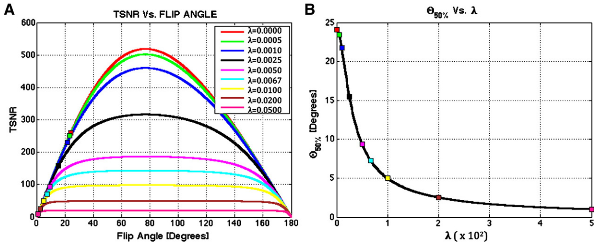
Fig. 2. (A) TSNR vs. Flip angle for T_1 = T_{1,GM} = 1.34 s, SNR_o = SNR_{o,GM} = 652 and different values of \lambda ranging from 0 to 0.05. For each curve, a square marks the angle below the Ernst angle for which TSNR has decreased to 50% from its maximum value ( \theta_{50\%} ). (B) Evolution of \theta_{50\%} with \lambda . The higher the amount of physiological noise present, the flatter the TSNR curve and consequently the lower the angle for which TSNR reaches 50% of its maximum value.
