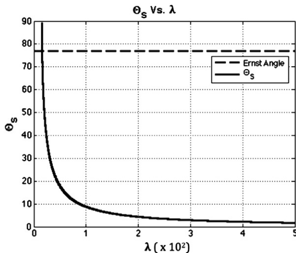
Fig. 4. Suggested flip angle ( \theta_S ) as a function of \lambda . The dotted line shows the Ernst angle for TR = 2 and T_1 = T_{1,GM} = 1.34 s. The continuous black line shows a plot of Eq. (10), the estimated \theta_S , as a function of \lambda while keeping SNR_o = SNR_{o,GM} = 652 .
